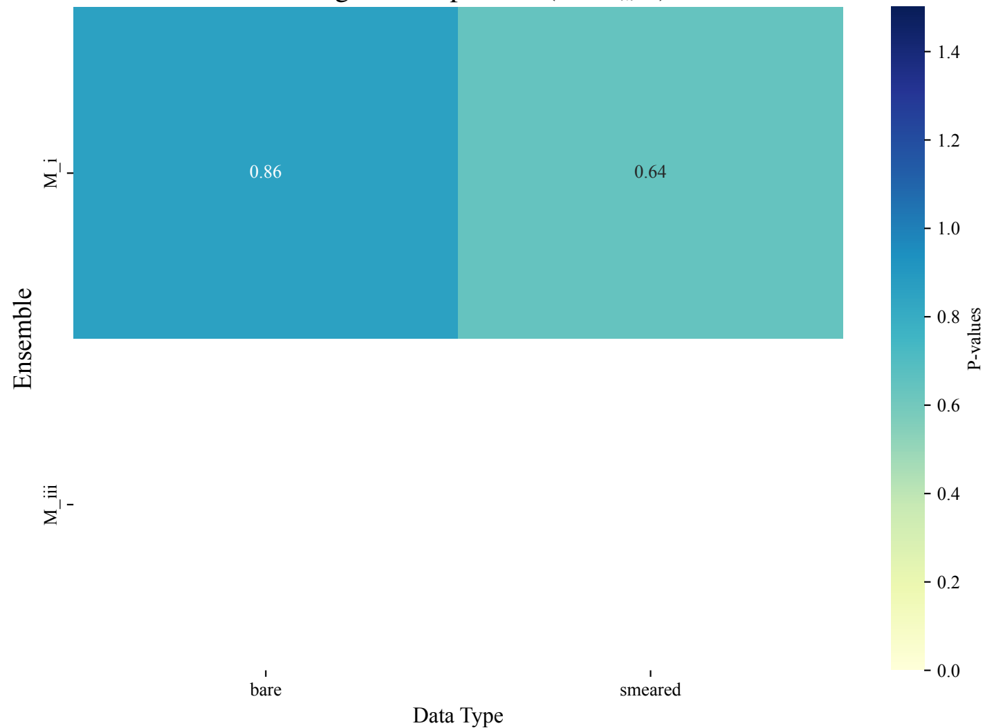
Full Log Model: p-value ( A = A_{\pi/12} )
